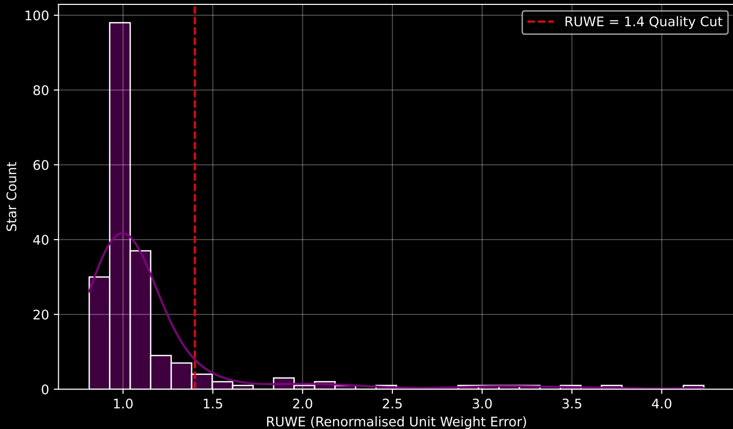
GAPOGEE DR17 Field [122+65_MGA] RUWE Distribution (n= 203)
