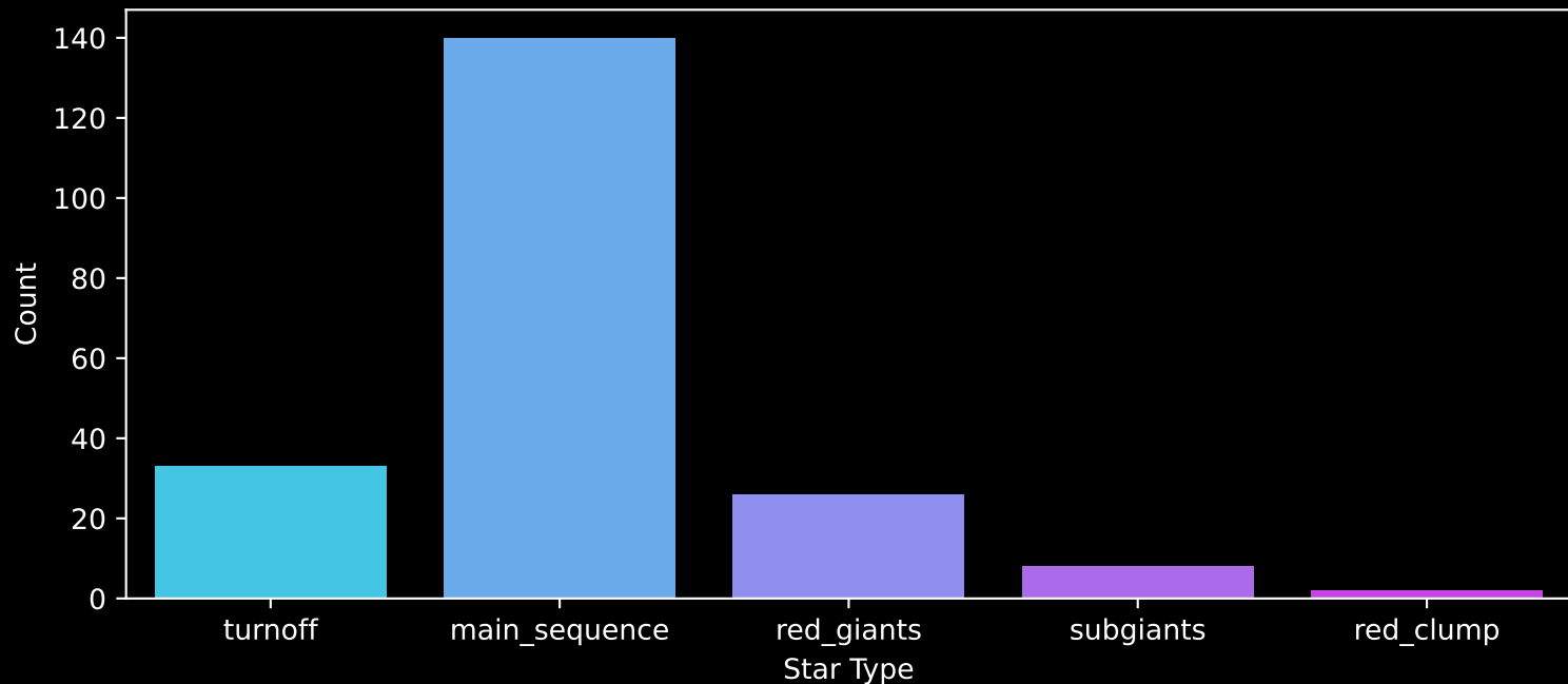
APOGEE DR17 Field: [122+65_MGA] Count plot of Star Type
