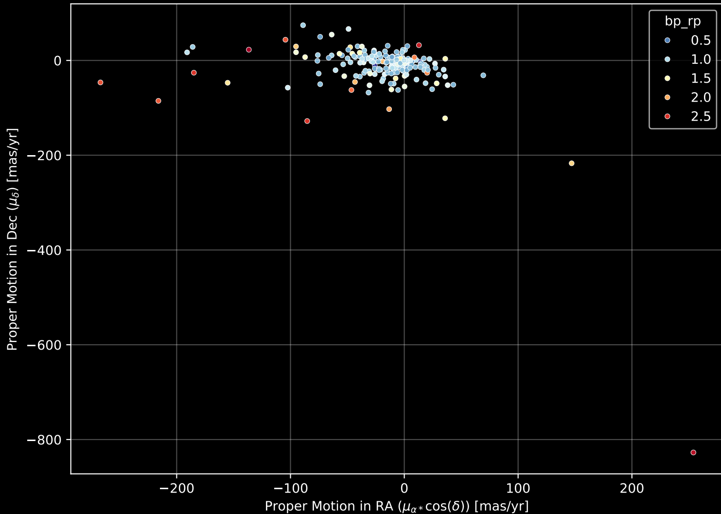
APOGEE DR17 Field: [122+65_MGA] Proper Motion Diagram (n= 209)
