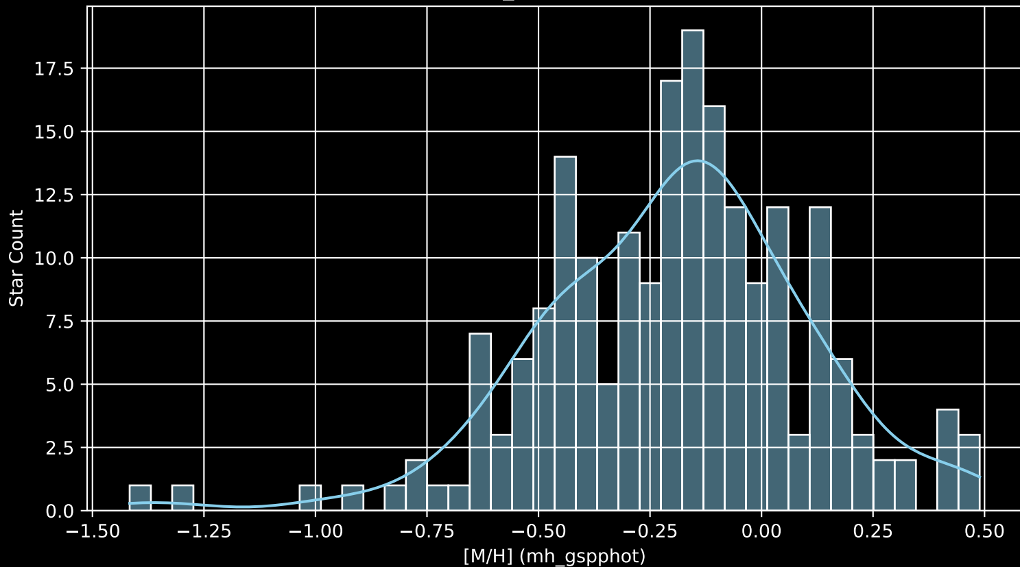
APOGEE DR17 Field: [122+65_MGA [M/H] (mh_gspphot) (n= 202)
