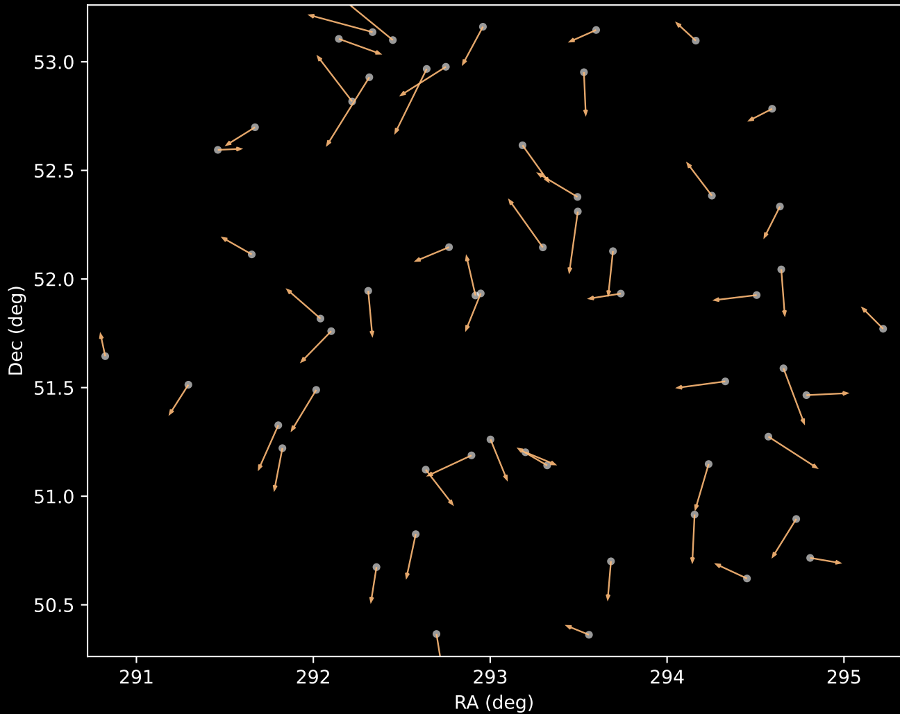
APOGEE DR17 Cluster 3 Proper Motion Vectors (n=56)
