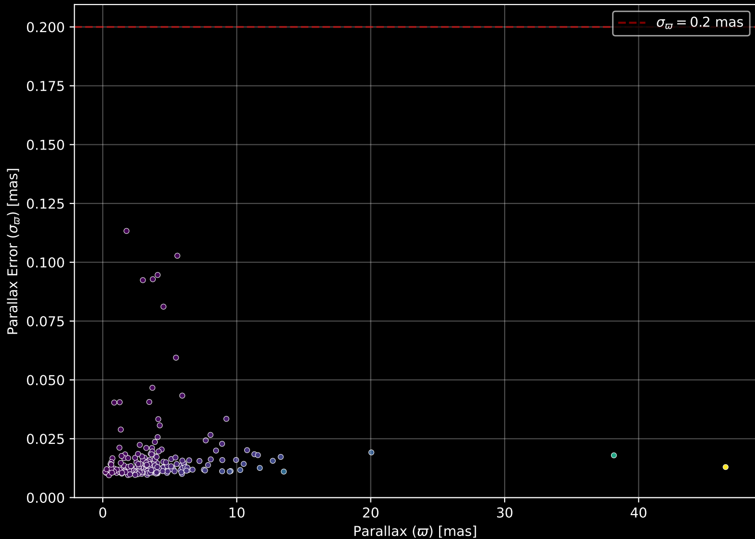
APOGEE DR17 Field: [122+65_MGA] Parallax Quality (n= 209)
