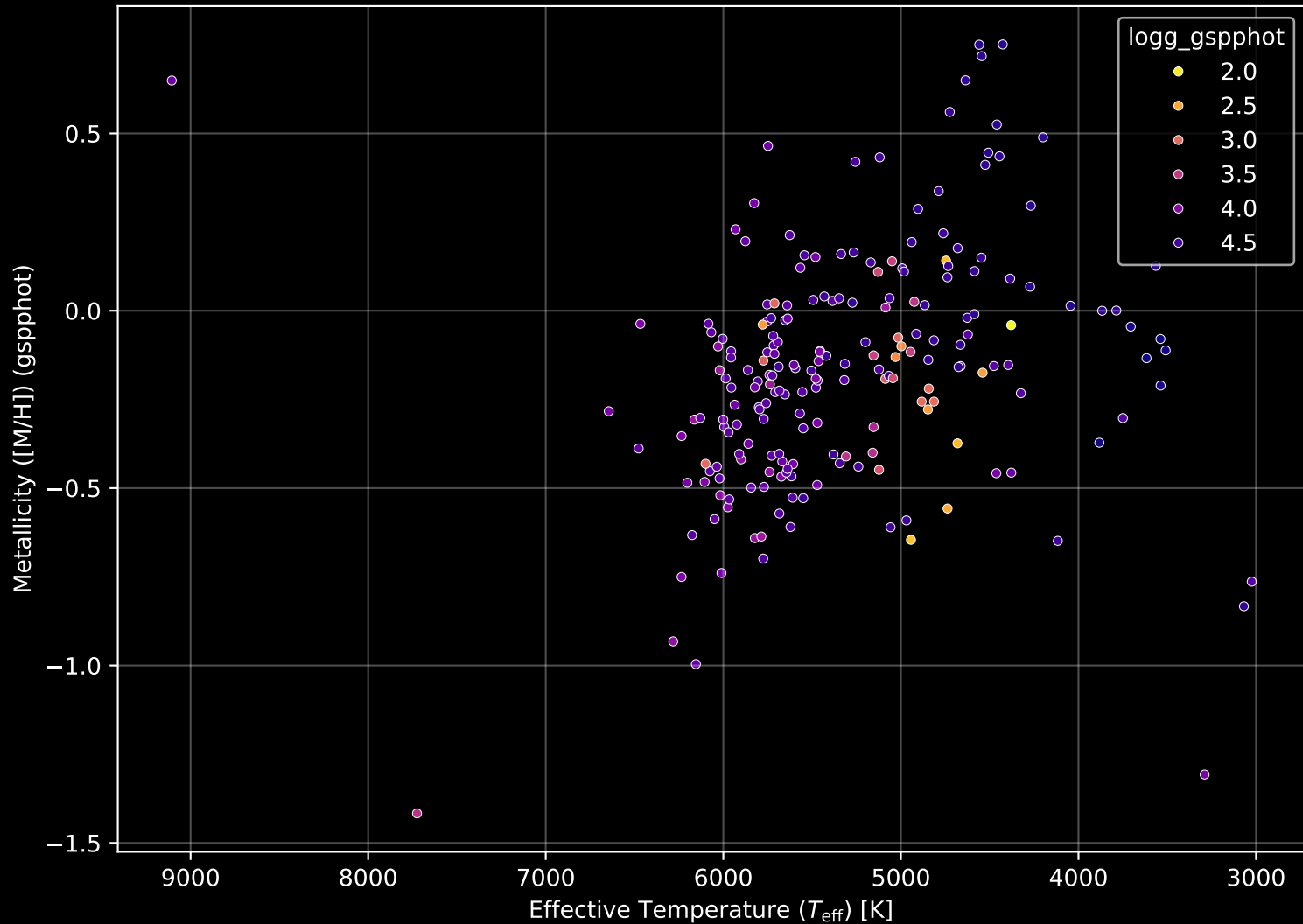
APOGEE DR17 Field: [122+65_MGA] Stellar Population Parameters (n= 209)
